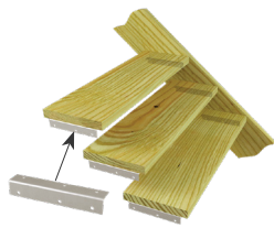
Typical SCA9-TZ installation
