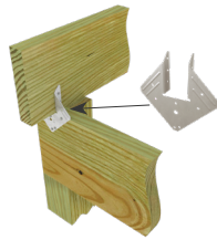
Typical RT15-TZ installation
