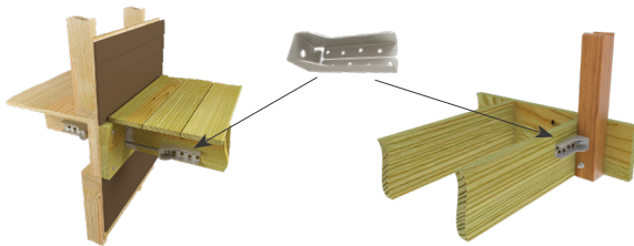
Typical DTB-TZ installations
