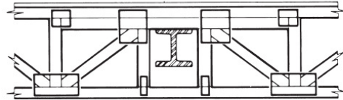
Intermediate Bearing - Floor Truss Supported by Steel or Wood Beam Special Engineering Required
