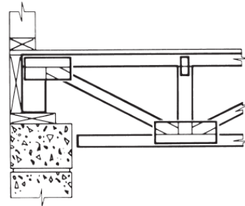
Top Chord Bearing on Masonry Wall
