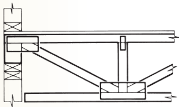
Top Chord Bearing on Frame Wall
