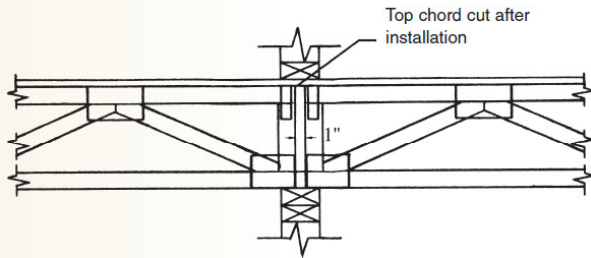
Intermediate Bearing - Simple Span Trusses
