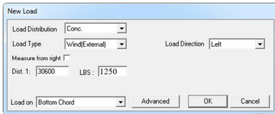
Figure 4 - Left Load
