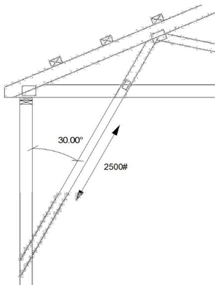
Figure 1 - Knee-Brace Diagram
